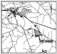
VICINITY MAP 1/28
